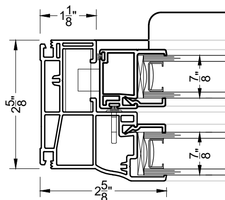
③ REPLACEMENT JAMB SH300
