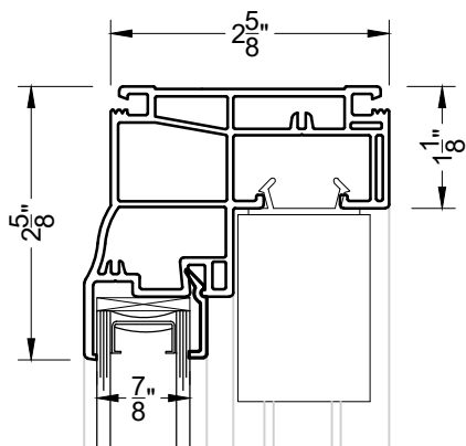
① REPLACEMENT HEAD SH300
