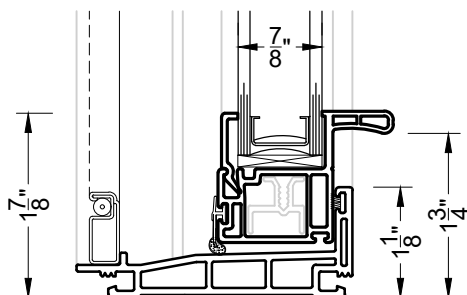
② REPLACEMENT SILL SH300
