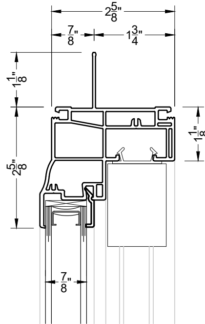
1 HEAD SH300
