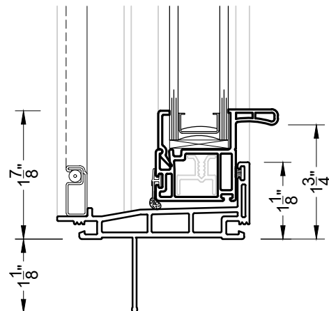
3 SILL SH300
