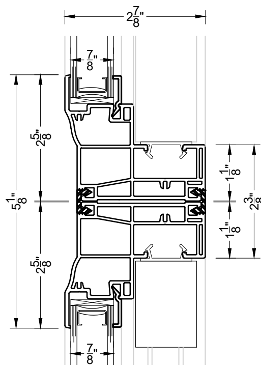
④ 0 DEGREE MULLION PW310 OVER SH300
